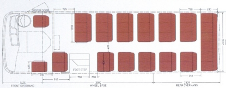
Double Door Option: Lynx 3900 - Seating capacity 34
