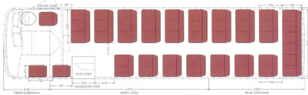
Lynx New-Look 4900 mm WB - 49 + D - Standard seats
