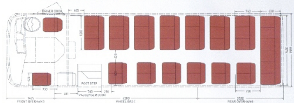
Double Door Option: Lynx 4200 - Seating capacity 39
